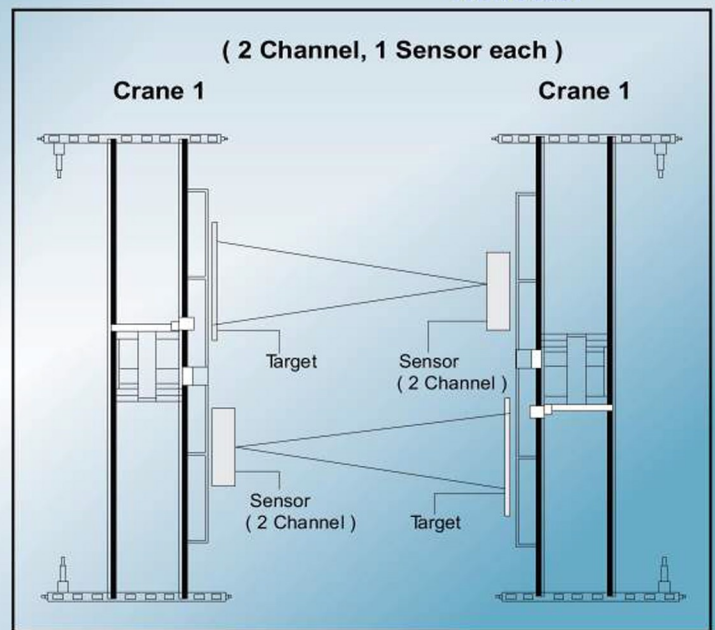
Cranes with Anti-collision System
