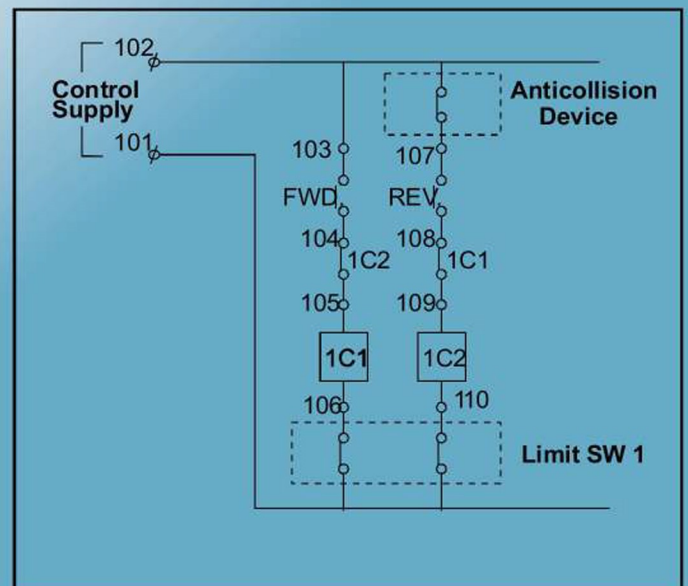
Cranes with Anti-collision System
